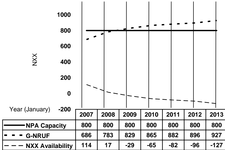
Figure 3 - NPA 418 CO Code Exhaust January 2007 R-NRUF
